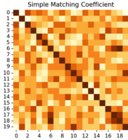
Fig. 10: Simple Matching Coefficient (SMC) heatmap
