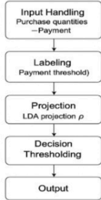
Fig. 2: Customer classification data flow
