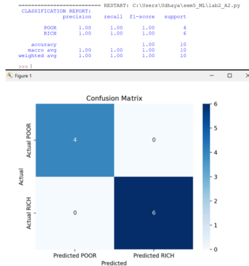
Fig. 6: Confusion matrix of RICH/POOR logistic regression classifier
