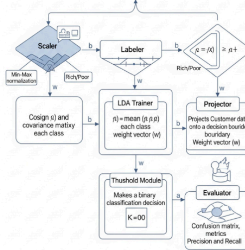
Fig. 4: Customer classification Architecture
